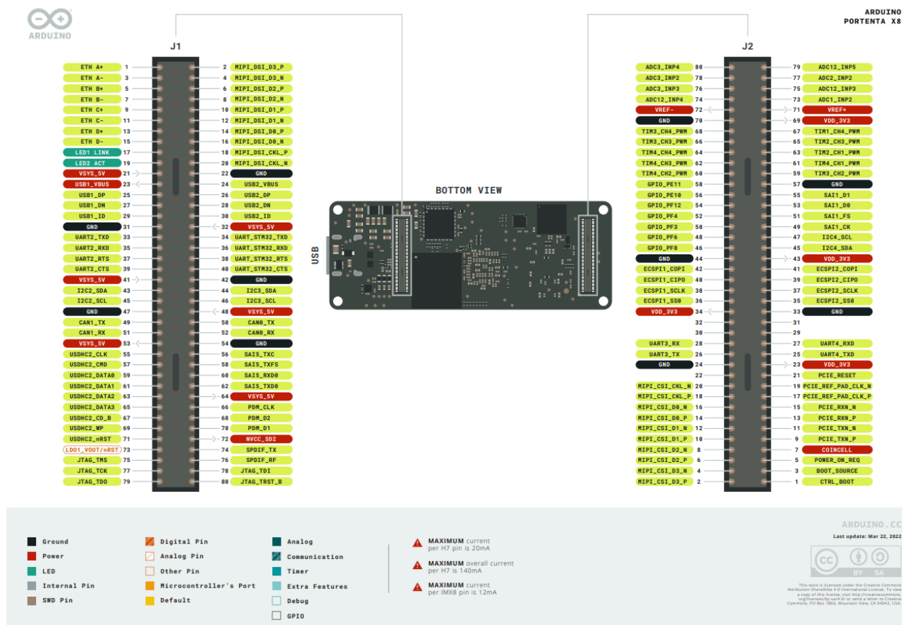
Figure 6. Portenta X8 High-Density connectors pinout
